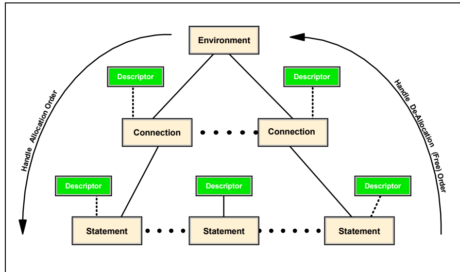
Figure 4-1 CLI handles
