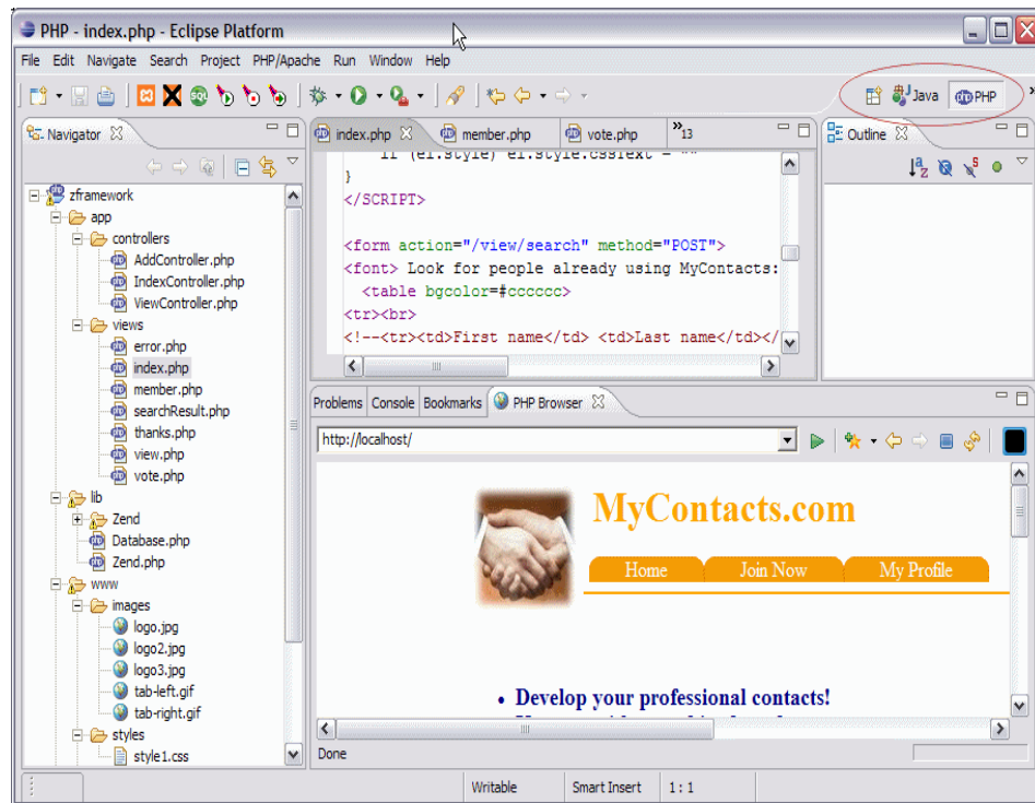
Figure 3-1 Eclipse
